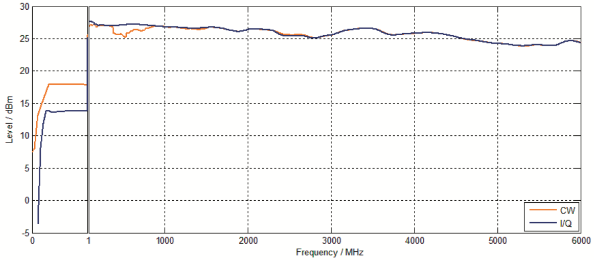
Maximum available output level versus frequency (meas.).
