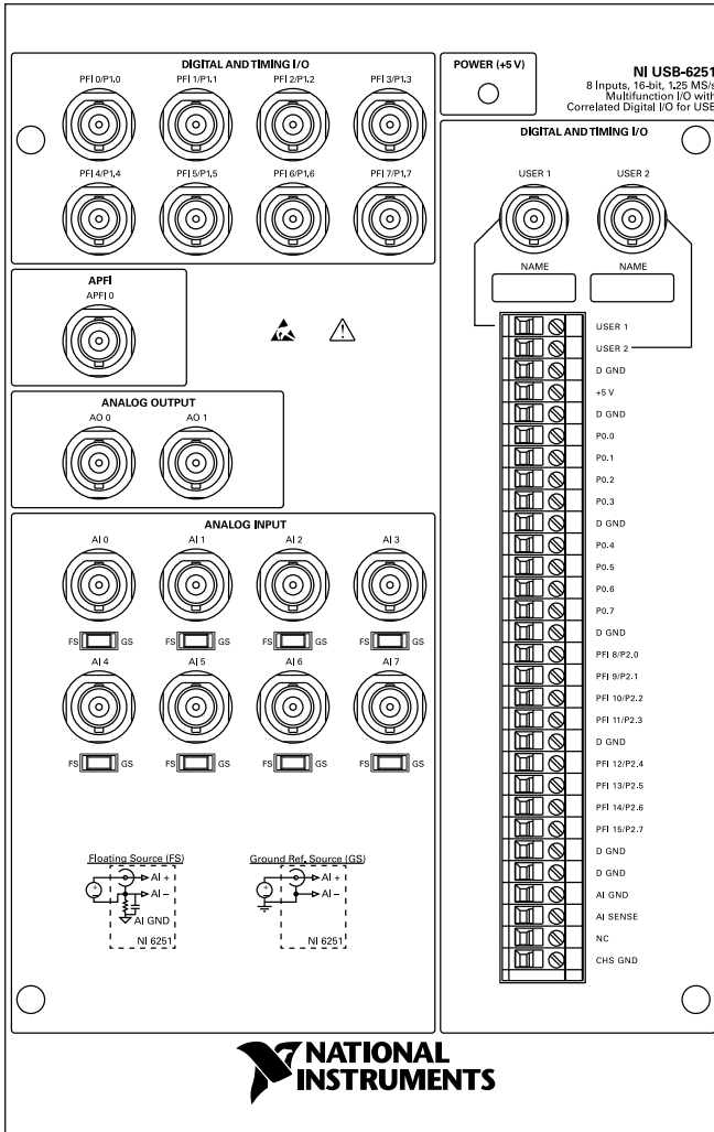
Figure 11. NI USB-6251 BNC Front Panel and Pinout
