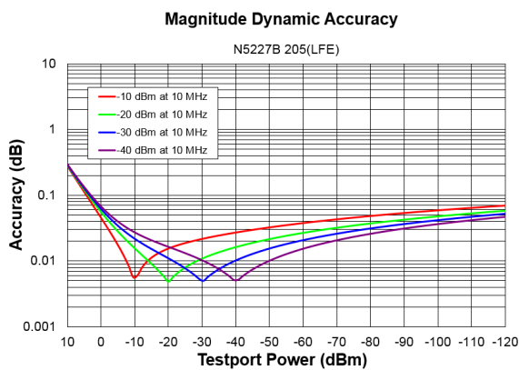
N5227B Dynamic Accuracy, 10 MHz, All LFE Options (LFE Enabled) - Specification
