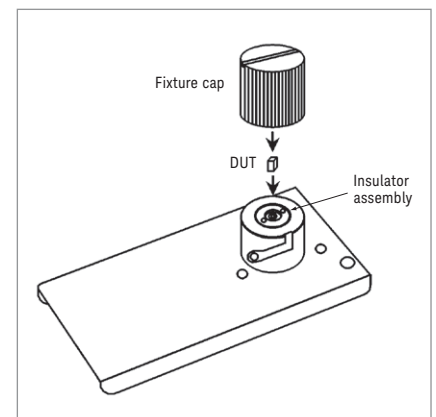
Figure 10. Positioning of the DUT
