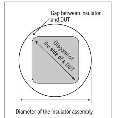
Figure 11. Gap between insulator and DUT
