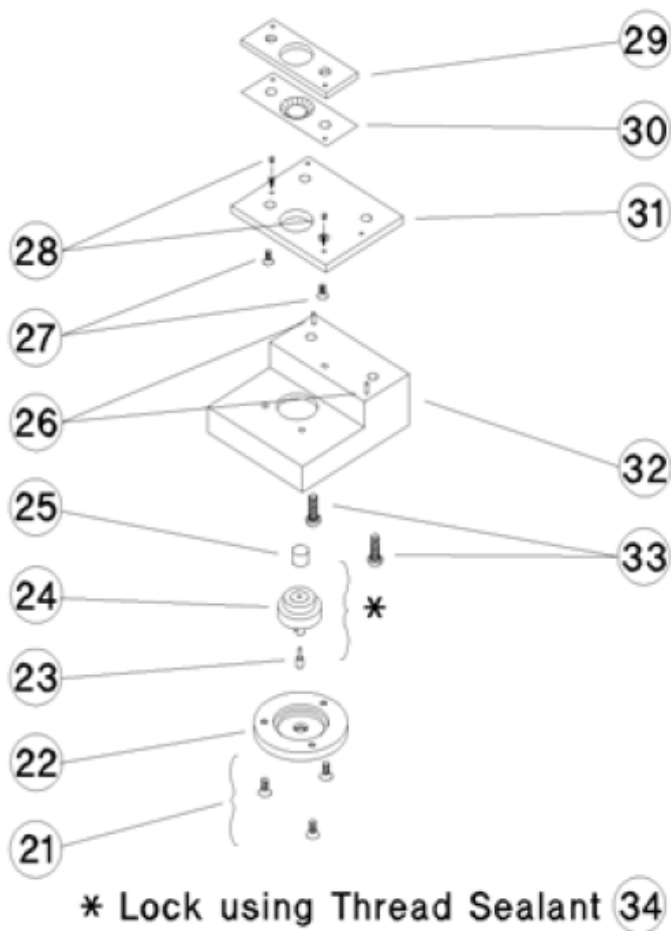
Replaceable Parts List (Lower Part)
