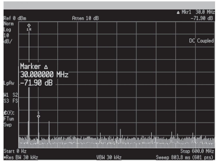
Figure 10. Spurious performance outstanding at low signal frequencies.
