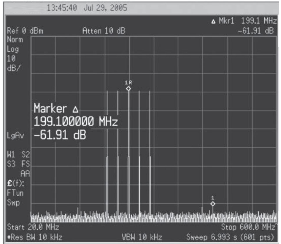
Figure 1. Generate wideband waveforms with unprecedented signal fidelity.
