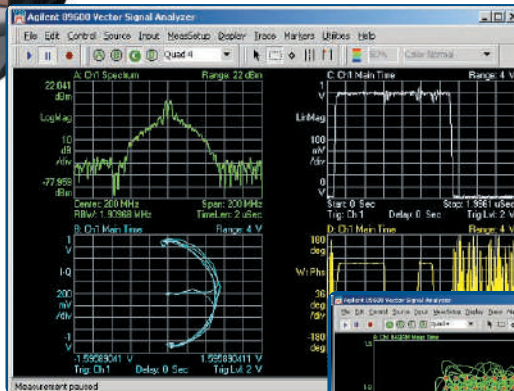
Barker coded radar pulse
