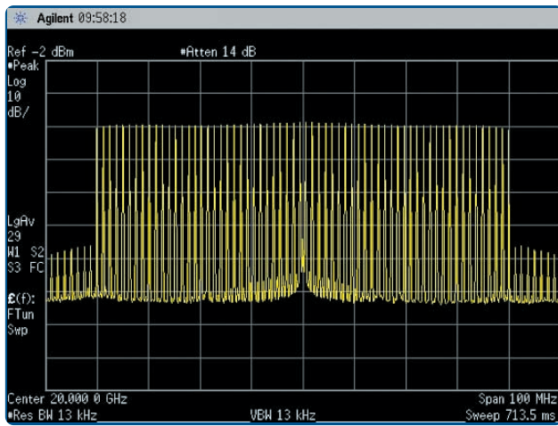
Multitone signal (64 tones generated)
