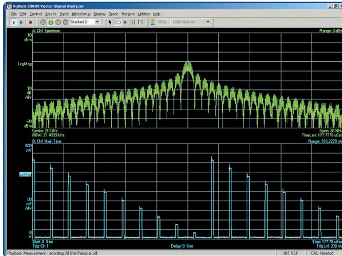
Custom pulse waveform created with MATLAB® and generated with the E8267C PSG
