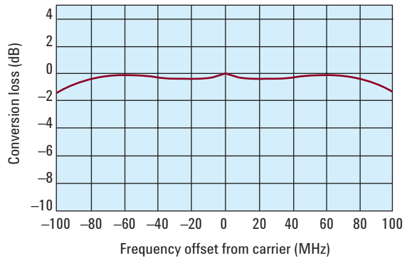
External I/Q modulation bandwidth (E8267C only)
