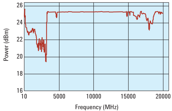
Typical maximum available power (all models)
