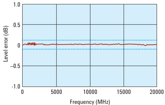
Typical level accuracy +5 dBm (all models)
