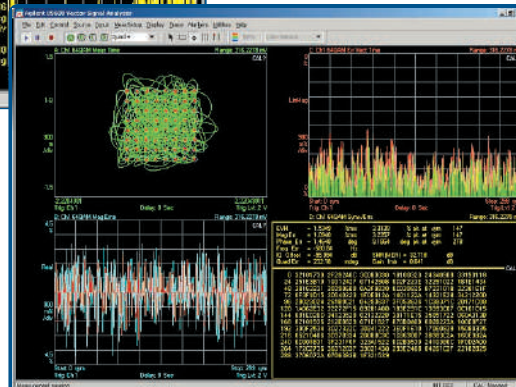
64 QAM signal at 20 GHz
