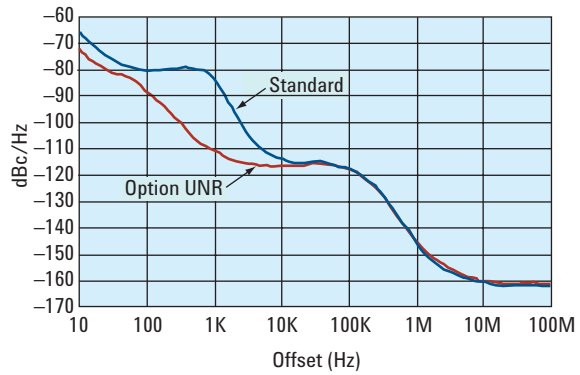
Standard and Option UNR phase noise at 10 GHz from 10 Hz to 100 MHz (all models)
