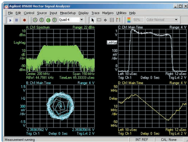
FM chirp radar pulse
