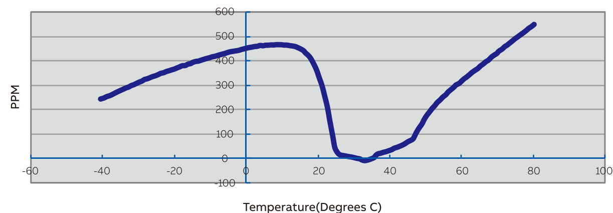
Phase Change vs Temperature(PPM)
