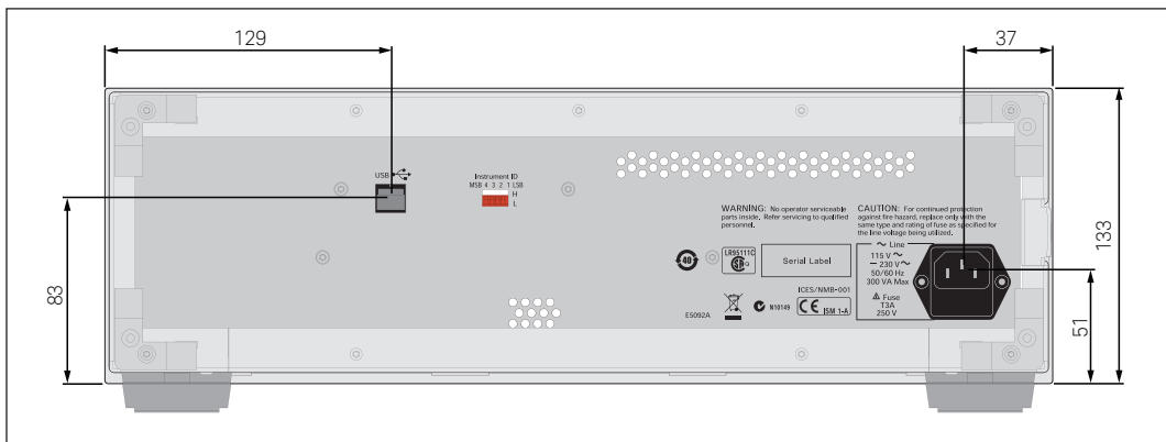
Figure 12. Dimensions (rear view, with Option E5092A-020, in millimeters, nominal)
