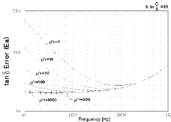
Figure 27. Permeability loss tangent ( \tan\delta ) accuracy vs. frequency (at F = 10 , typical) 1
