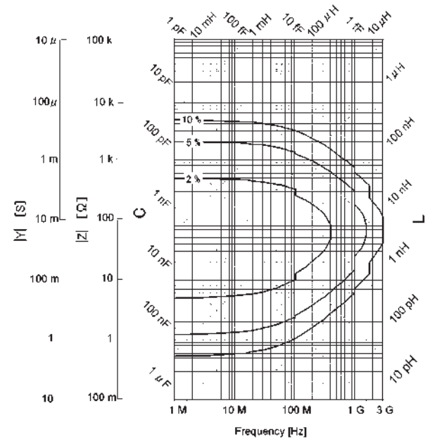
Figure 4. |Z| , |Y| Measurement accuracy when open/short/load calibration is performed. Oscillator level < -33 dBm within \pm 5 °C from the calibration temperature.
