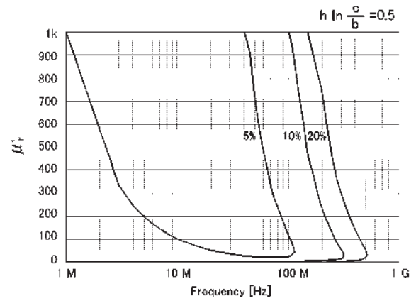
Figure 51. Permeability ( \mu' ) vs. frequency (at F = 0.5 , typical)
