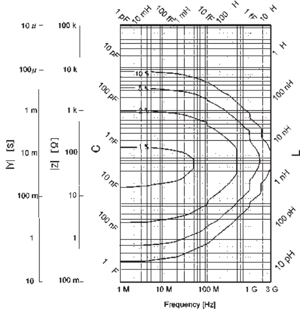
Figure 31. |Z| , |Y| measurement accuracy when open/short/load calibration is performed. Oscillator level = -23 dBm, -13 dBm, -3 dBm. Point averaging factor \geq 8 within \pm 5^\circ\text{C} of calibration temperature.
