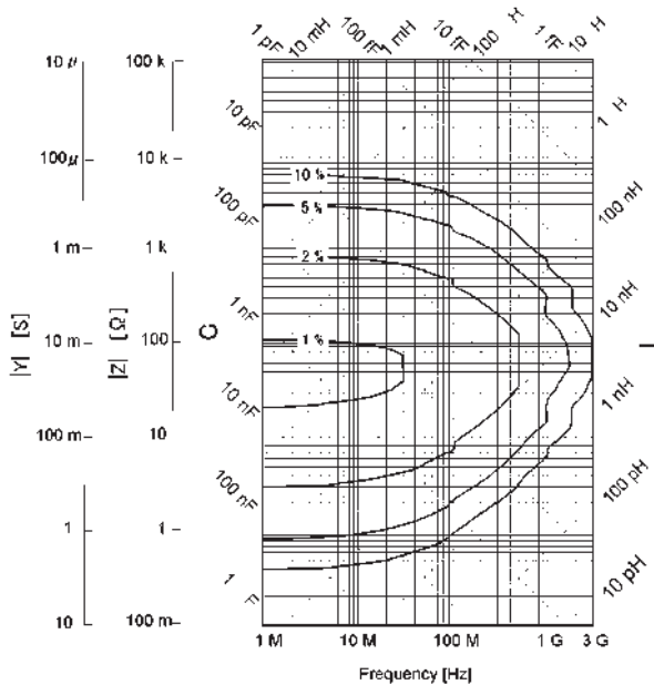
Figure 32. |Z| , |Y| measurement accuracy when open/short/load calibration is performed. Oscillator level \geq -33 dBm. Point averaging factor \geq 8 within \pm 5^\circ\text{C} of calibration temperature.
