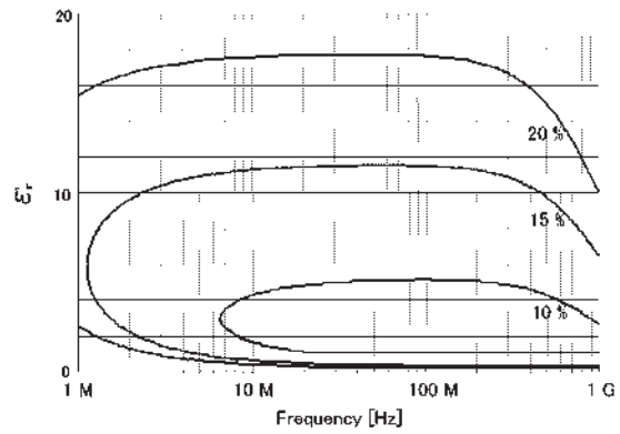
Figure 19. Permittivity ( \epsilon_p' ) vs. frequency (at t = 0.3 mm, typical)
