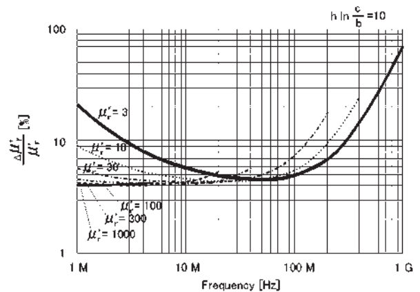
Figure 24. Permeability accuracy \left(\frac{\Delta\mu'}{\mu'}\right) vs. frequency (at F = 10 , typical)
