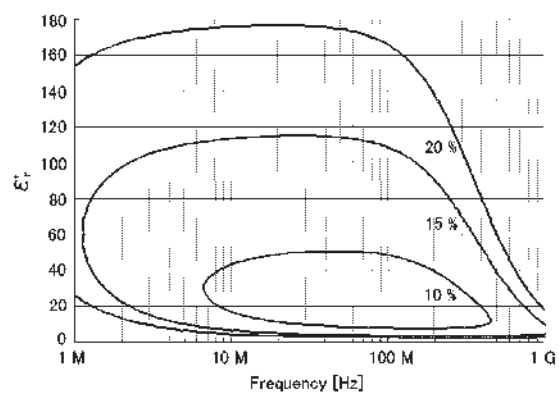
Figure 21. Permittivity ( \epsilon_p' ) vs. frequency (at t = 3 mm, typical)
