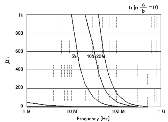
Figure 53. Permeability ( \mu' ) vs. frequency (at F = 10 , typical)
