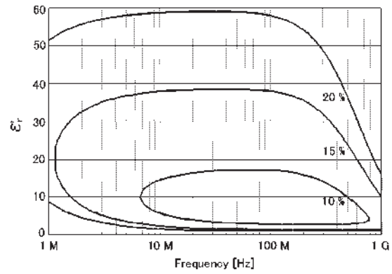
Figure 20. Permittivity ( \epsilon_p' ) vs. frequency (at t = 1 mm, typical)
