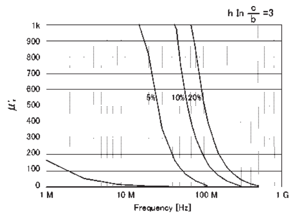
Figure 52. Permeability ( \mu' ) vs. frequency (at F = 3 , typical)
