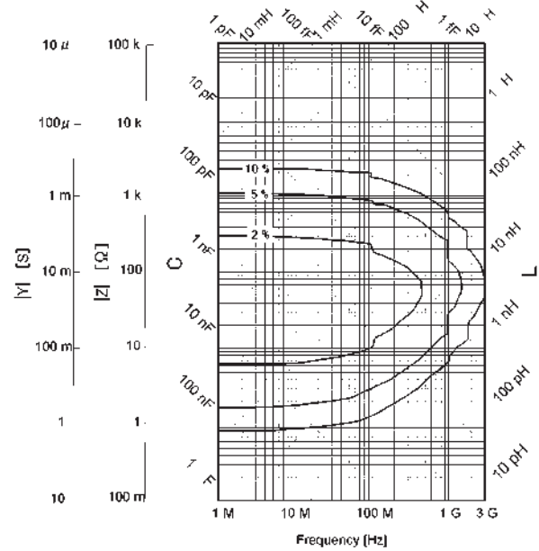
Figure 33. |Z| , |Y| measurement accuracy when open/short/load calibration is performed. Oscillator level \geq -33 dBm. Point averaging factor \leq 7 within \pm 5^\circ\text{C} of calibration temperature.
