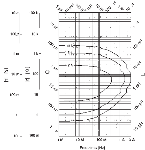
Figure 34. |Z| , |Y| measurement accuracy when open/short/load calibration is performed. Oscillator level < -33 dBm. Point averaging factor \geq 8 within \pm 5^\circ\text{C} of calibration temperature.
